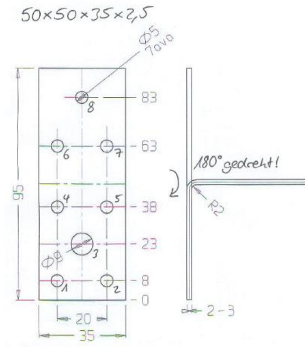
Figure A. 1 Dimensions of angle bracket 50x50x35x2,5
