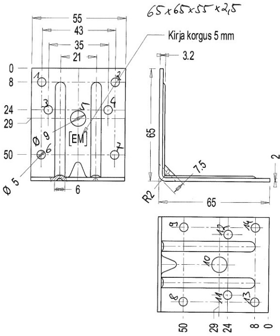
Figure B. 33 Dimensions of angle bracket 65x65x55x2,5
