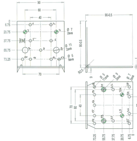
Figure B. 59 Dimensions of angle bracket
