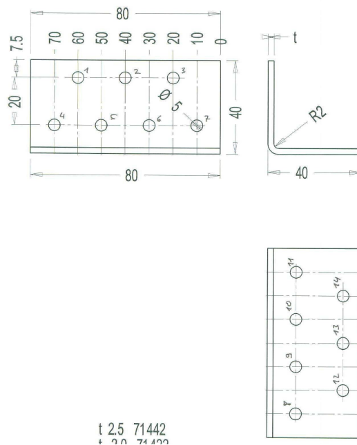
Figure B. 8 Dimensions of angle bracket
