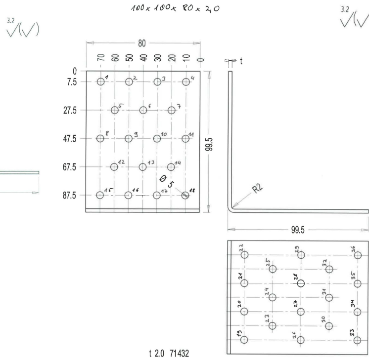
Figure B. 69 Dimensions of angle bracket
