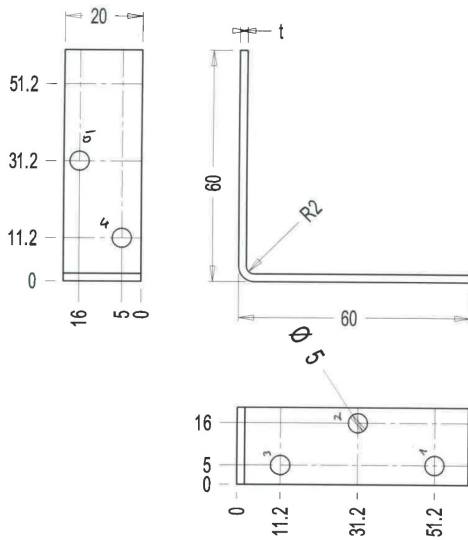
Figure B. 16 Dimensions of angle bracket
