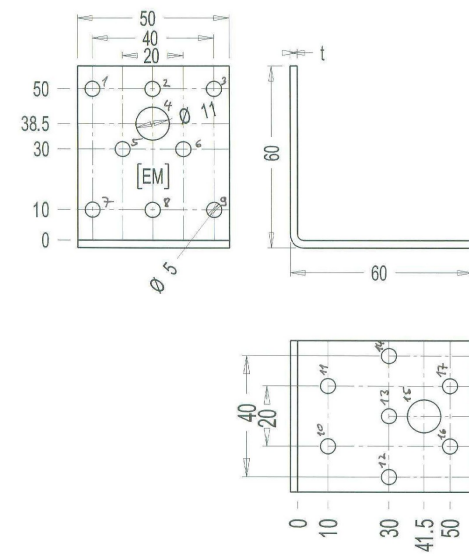
Figure B. 21 Dimensions of angle bracket
