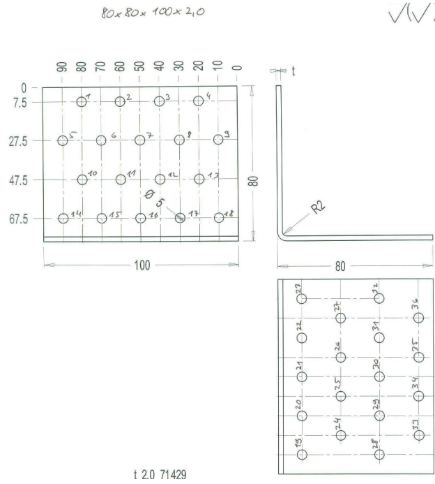
Figure B. 45 Dimensions of angle bracket
