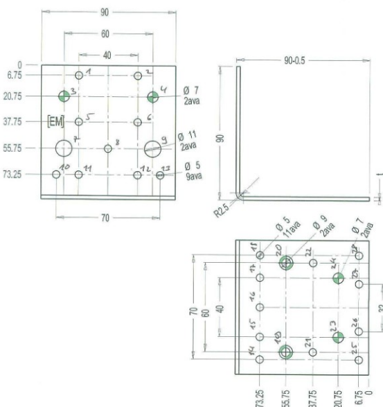
Figure B. 58 Dimensions of angle bracket
